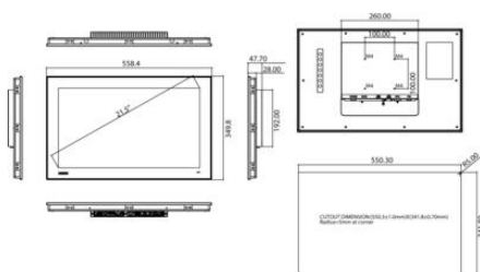
Panel Cut-out Dimensions: 550.30 x 341.8 mm (21.67" x 13.46")
