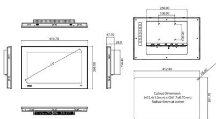
Panel Cut-out Dimensions: 412.40 x 261.70 mm (16.24" x 10.30")
