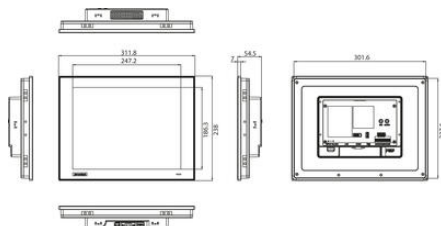
Panel Cut-out Dimensions: 302.5 x 228.5 mm (12.1" x 9.14")
