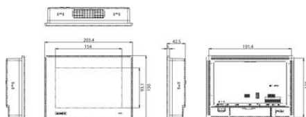
Panel Cut Out Dimensions: 192 x 138.5 mm (7.56" x 5.45")
