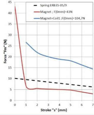
Force-stroke curve(F-S)
