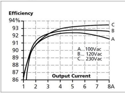
Fig. 9-1 Efficiency vs. output current at 30V, typ.
