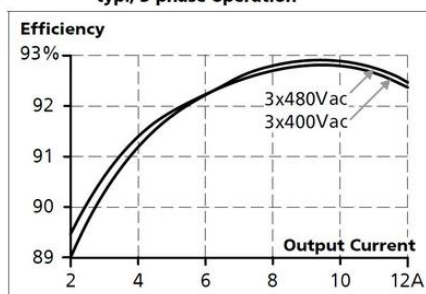
Fig. 8-1 Efficiency vs. output current at 24V, typ., 3-phase operation
