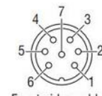
Front side molded 7P Female connector
