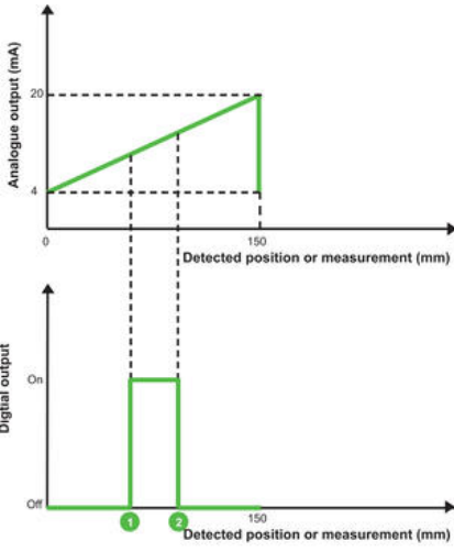
1 } Detection order of the switching interval extremes 2 }
